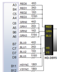
Artix-7
